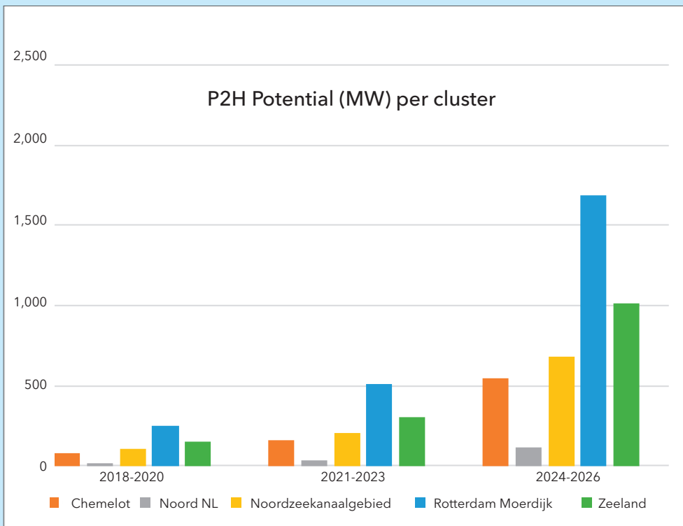
Figure 10 - Development in time of the P2H power for the five industry clusters in the Netherlands
