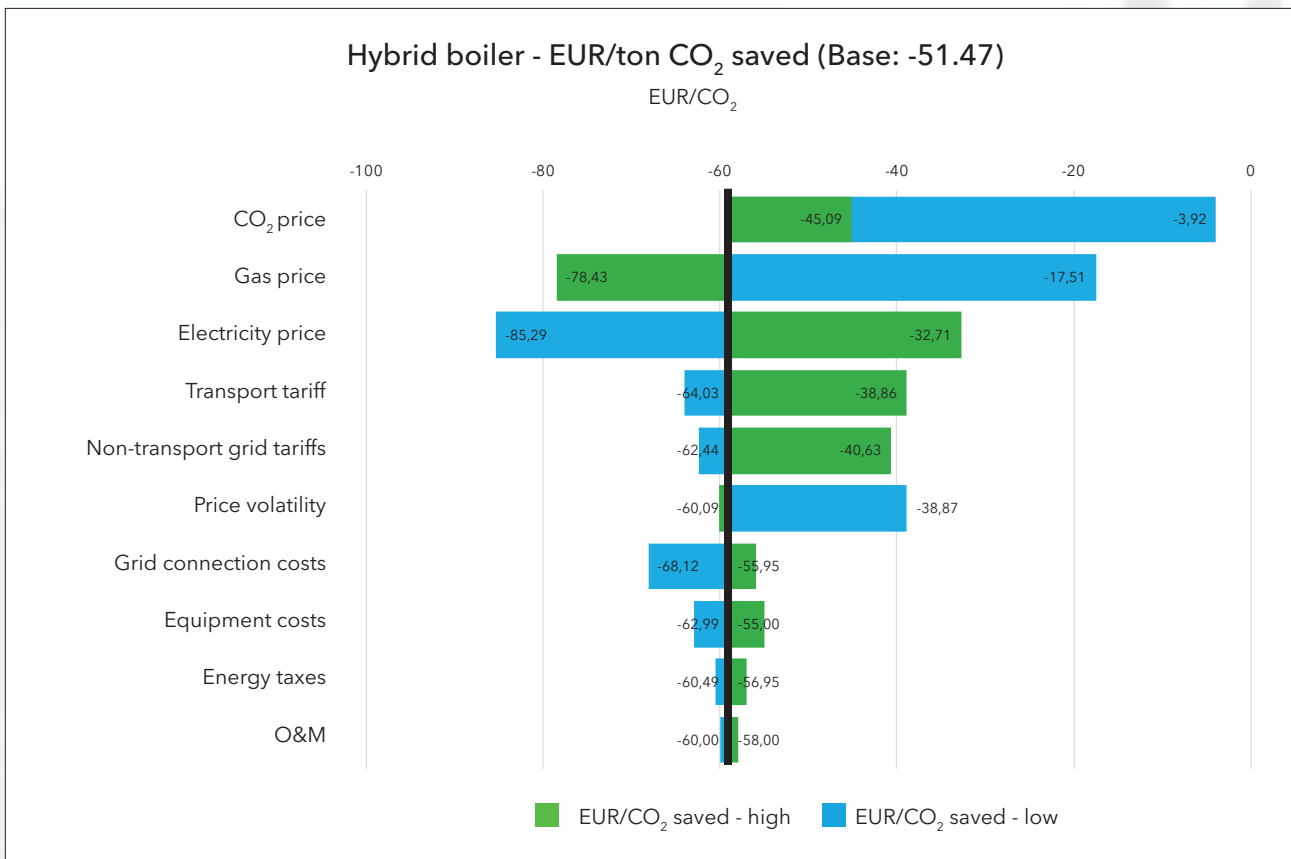
Figure 17 - EUR/ton CO 2 saved sensitivity
