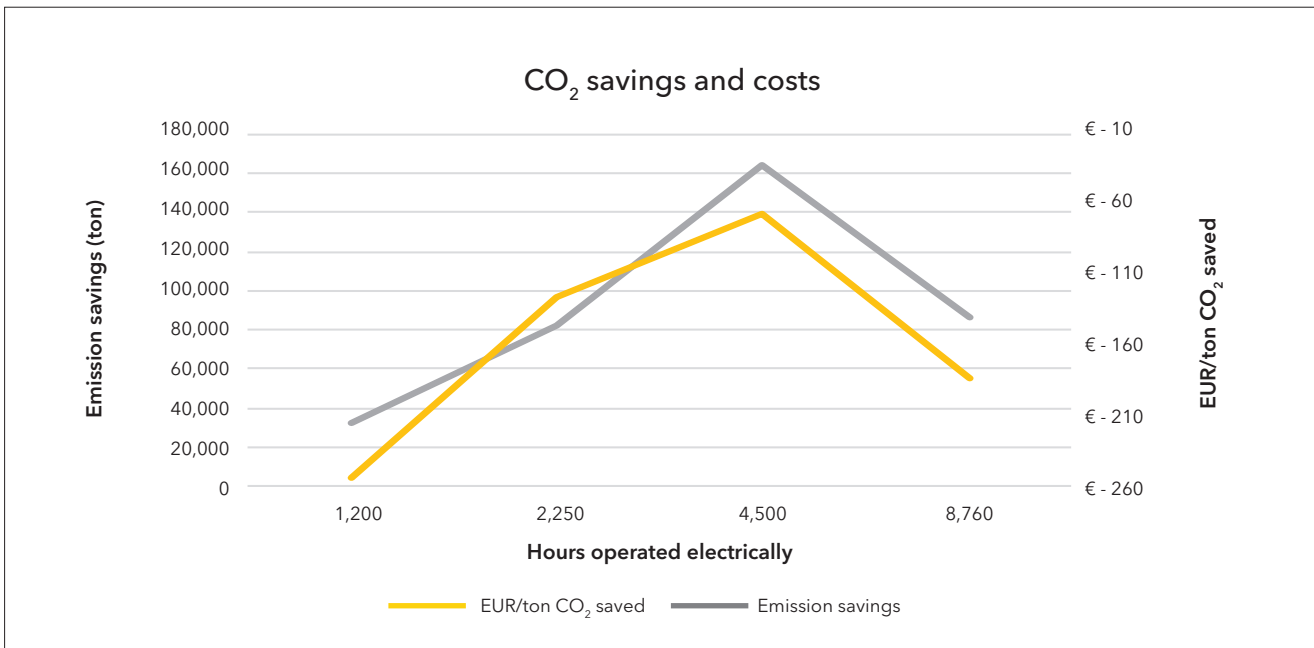
Figure 15 - Overview of emission savings and emission savings costs for the different operating scenarios
