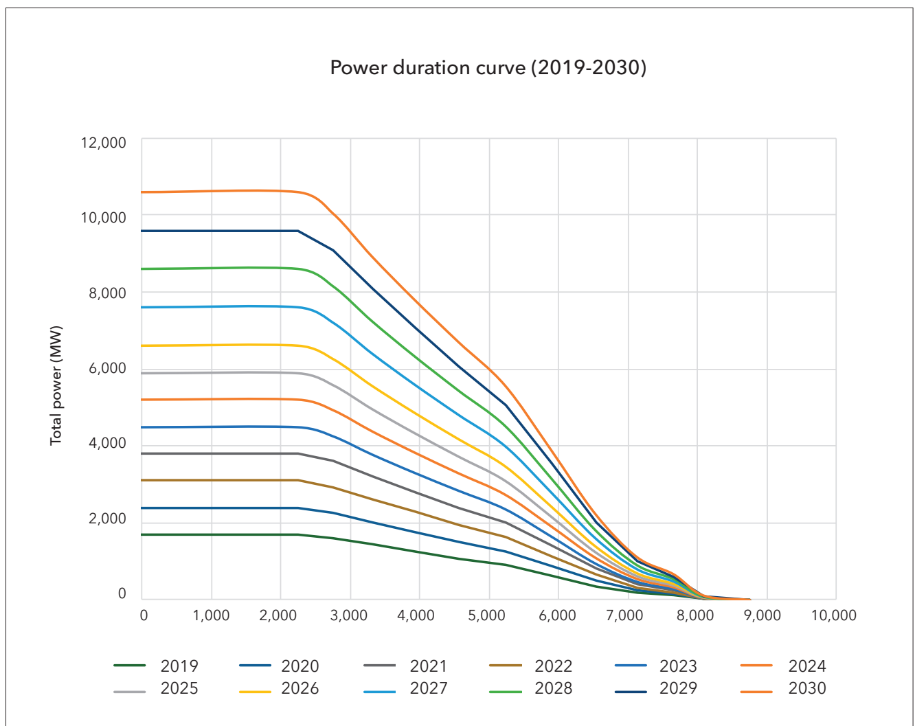
Figure 8 - The power duration curves for the installed offshore wind farms over the years
