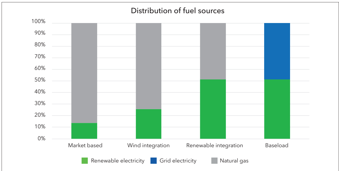
Figure 14 - Distribution of fuel source per scenario
